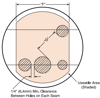
Three Section End Plate
